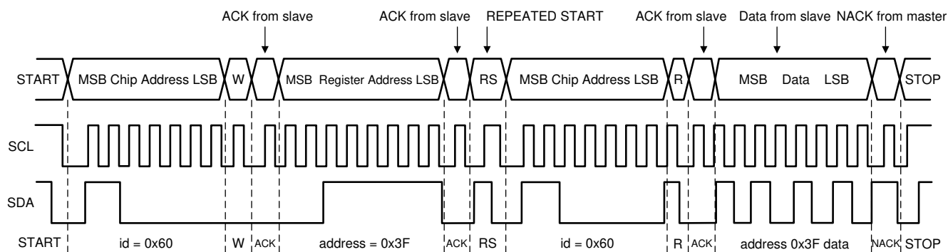
图 7-20. Read Cycle (r = read; SDA = 1). Example Device Address = 0x60
