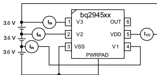
图 8-3. Configuration for IC Current Consumption Test
