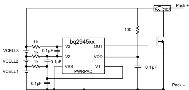
图 9-4. 3-Series Cell Configuration with Fixed Delay
