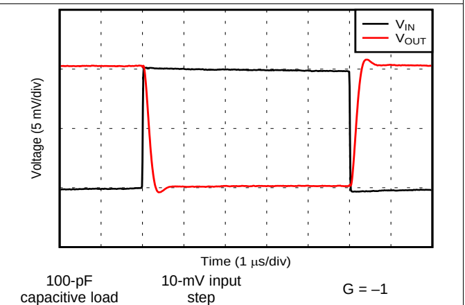
图 30. Small-Signal Step Response
