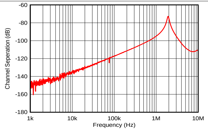
图 26. Channel Separation vs Frequency
