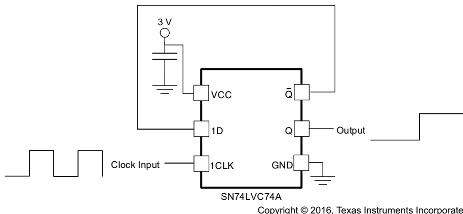
Figure 4. Frequency Divider
