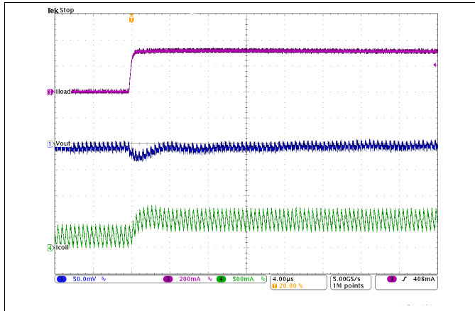
Figure 24. Load Transient Response in PWM Mode, Rising Edge
