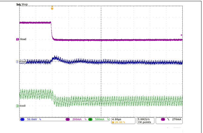
Figure 25. Load Transient Response in PWM Mode, Falling Edge
