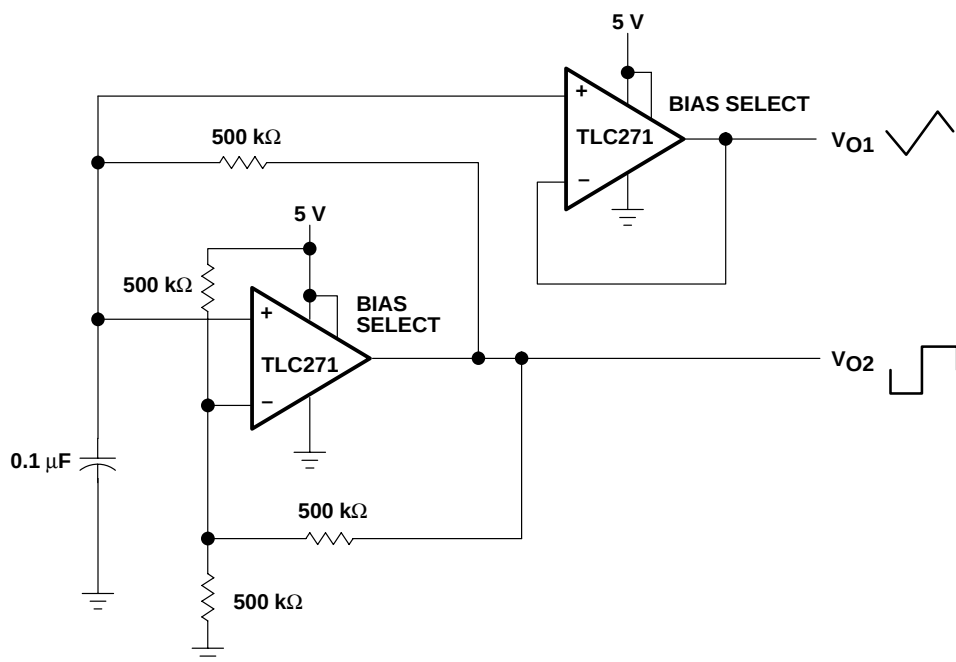
Figure 126. Multivibrator
