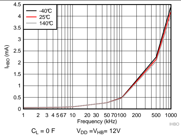
图 5. HB Operating Current
