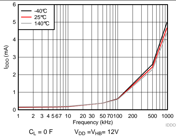
图 4. VDD Operating Current
