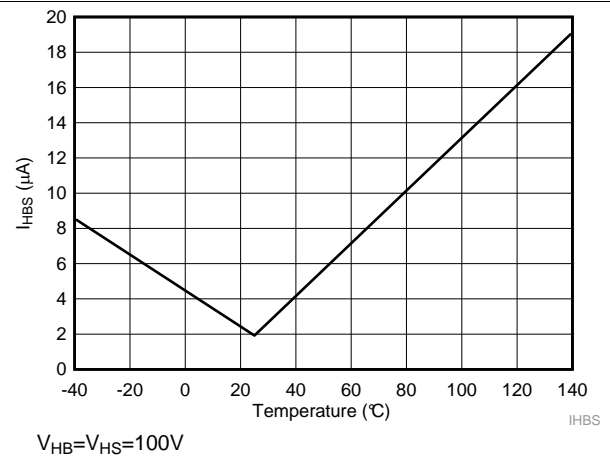
图 7. HB to VSS Quiescent Current
