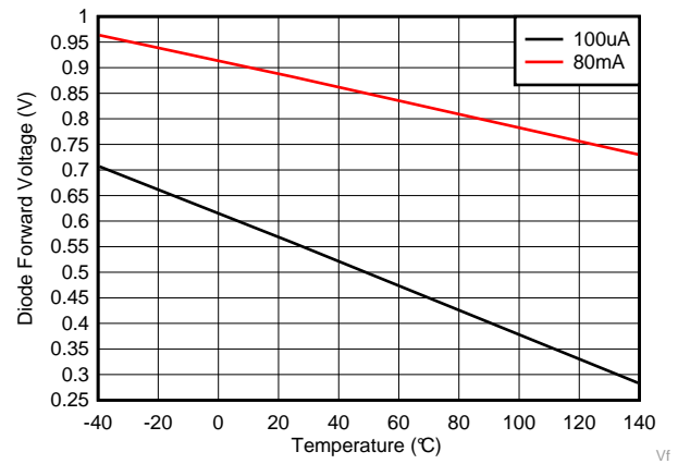
图 17. Boot Diode Forward Voltage Drop
