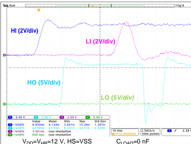
图 42. Input Shoot-through Protection or Interlock
