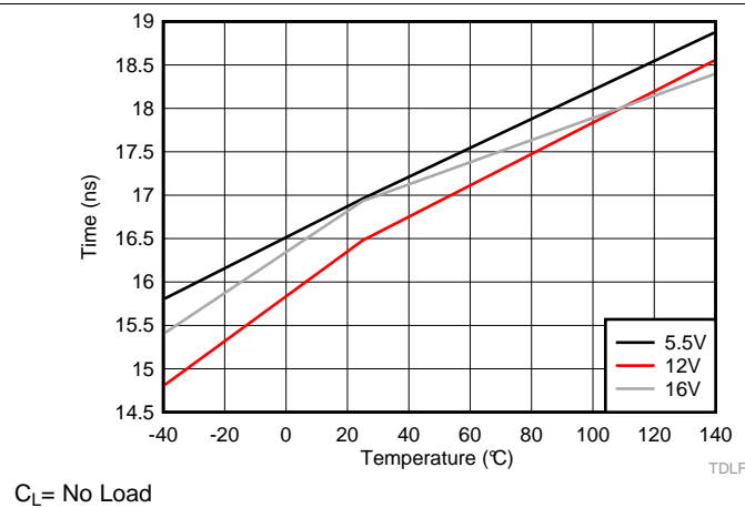
图 32. LO Falling Propagation Delay (TDLFF)
