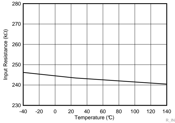
图 10. Input Pull-down Resistor
