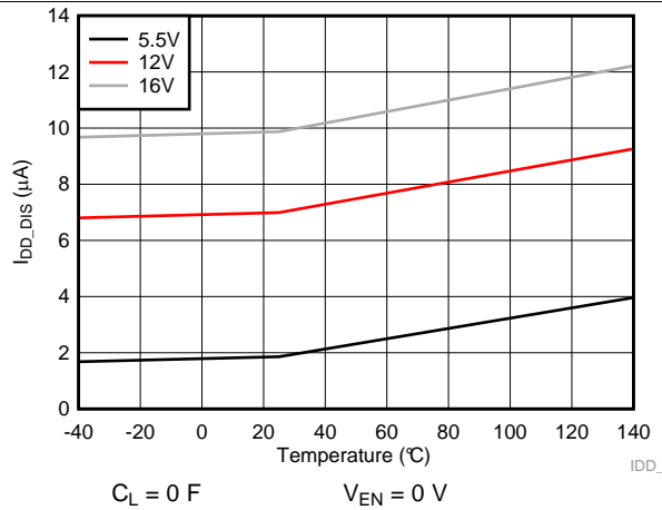
图 6. VDD Current When Disabled
