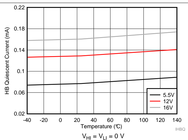
图 3. HB Quiescent Current
