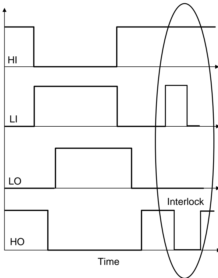
图 33. Interlock or Input Shoot-through Protection
