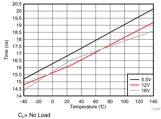
图 30. HO Falling Propagation Delay (TDHFF)
