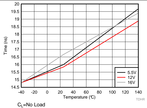
图 29. HO Rising Propagation Delay (TDHRR)
