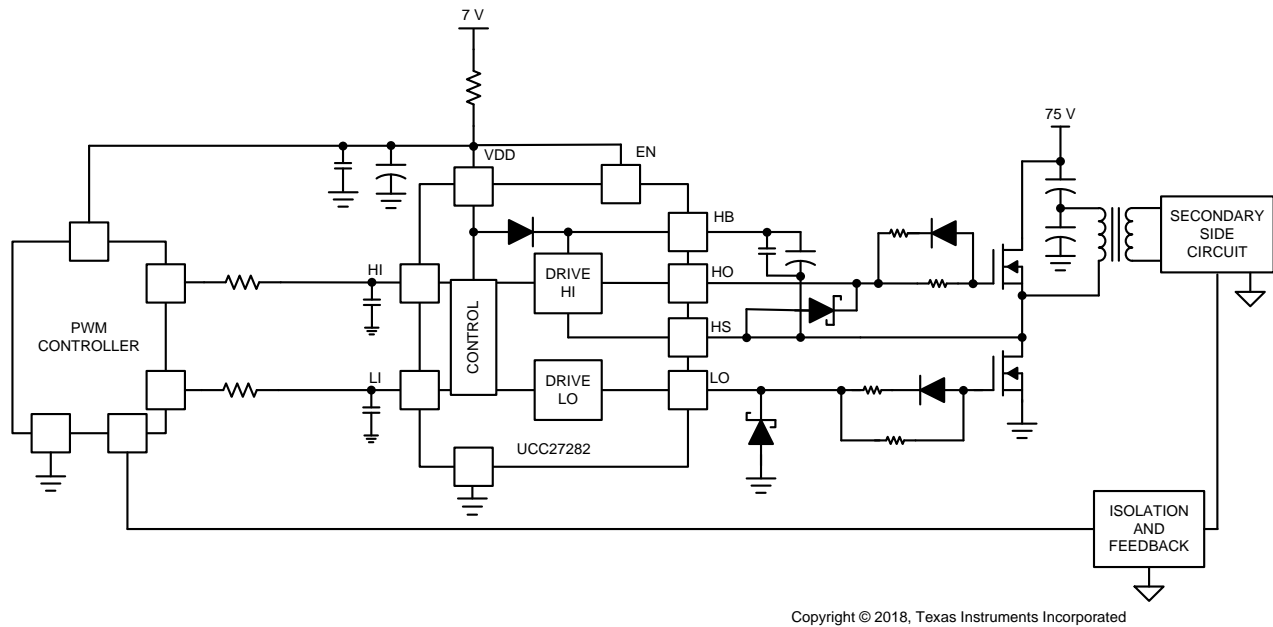
图 34. Typical Application
