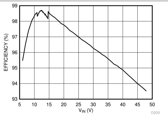
图 8-3. Efficiency vs Input Voltage
