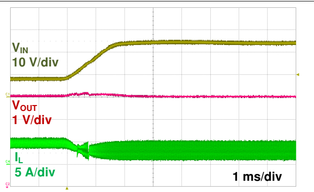
图 8-5. Line Transient Response (8 V - 24 V, IOUT = 2 A)
