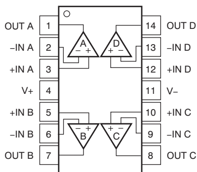
Pin Functions: MCP6294
