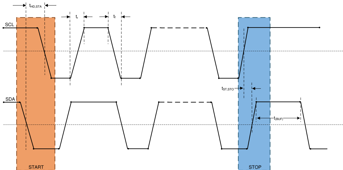
图 13. Start and Stop Condition Timing
