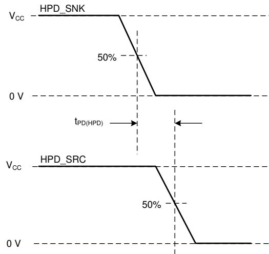
图 11. HPD Timing Diagram No. 1
