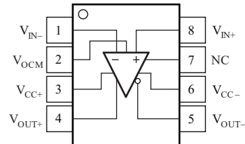
Figure 6-2. D, DGN, or DGK Package 8-Pin SOIC, MSOP, or MSOP-PowerPAD THS4131 Top View
