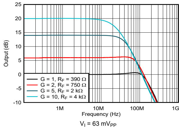
Figure 7-1. Small-Signal Frequency Response
