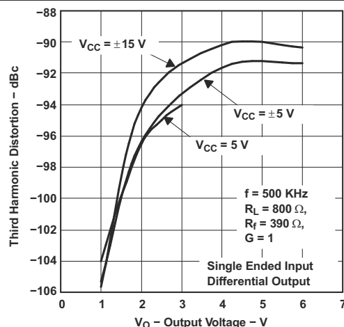
Figure 7-50. Third-Harmonic Distortion vs Output Voltage
