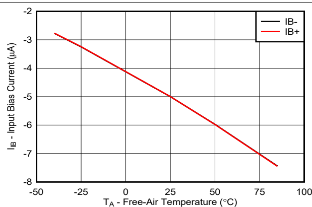
Figure 7-11. Input Bias Current vs Free-Air Temperature
