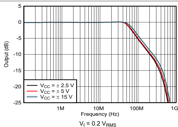
Figure 7-7. Large-Signal Frequency Response
