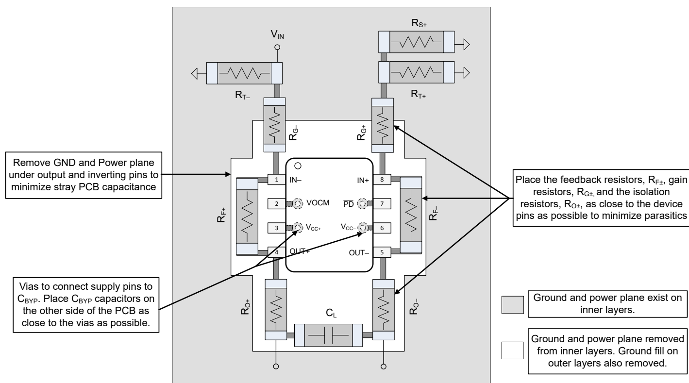
Figure 11-2. Layout Recommendations
