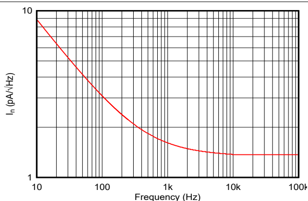
Figure 7-25. Current Noise vs Frequency
