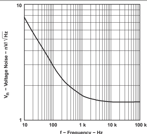
Figure 7-52. Voltage Noise vs Frequency
