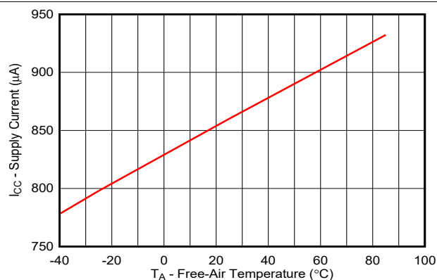
Figure 7-10. Supply Current vs Free-Air Temperature (Shutdown State)
