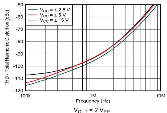
Figure 3-2. Total Harmonic Distortion vs Frequency
