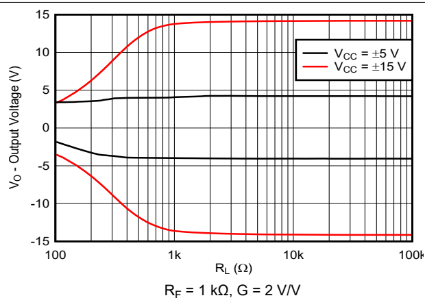
Figure 7-27. Output Voltage vs Differential Load Resistance R_F = 1\text{ k}\Omega , G = 2\text{ V/V}
