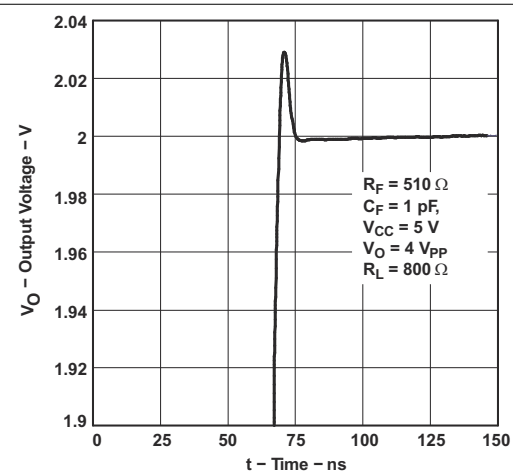
Figure 7-40. Settling Time
