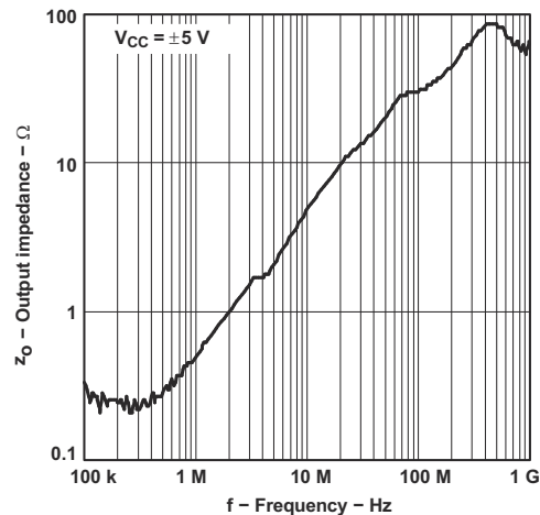
Figure 7-56. Output Impedance vs Frequency
