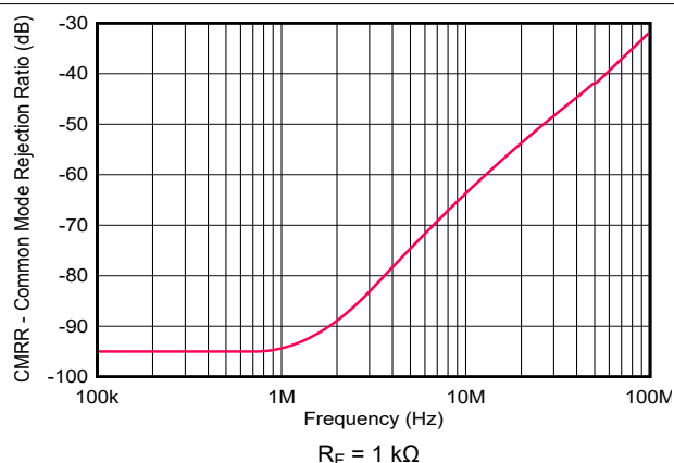
Figure 7-8. Common-Mode Rejection Ratio vs Frequency
