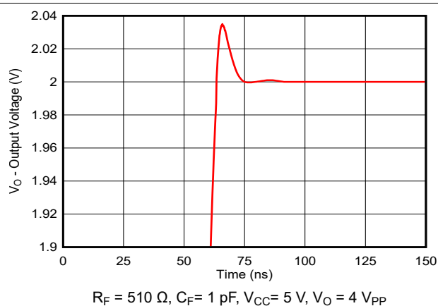
Figure 7-12. Settling Time
