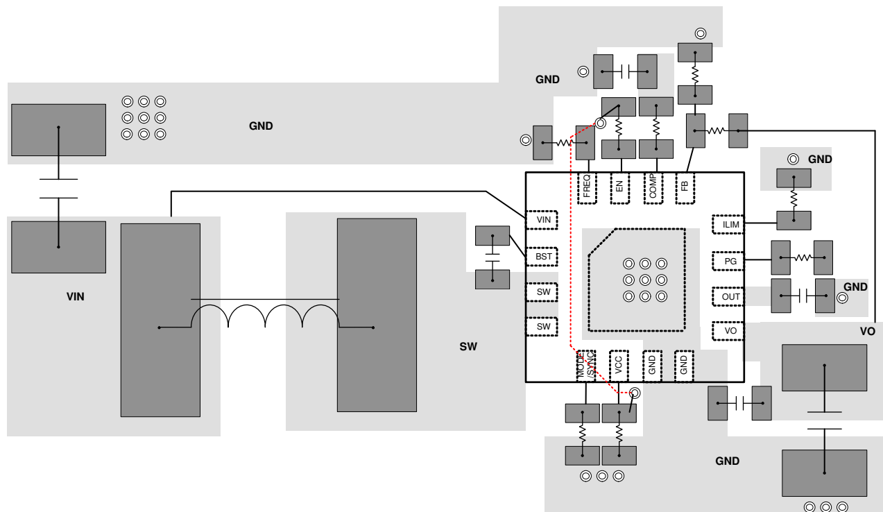
图 11-1. Recommended Layout
