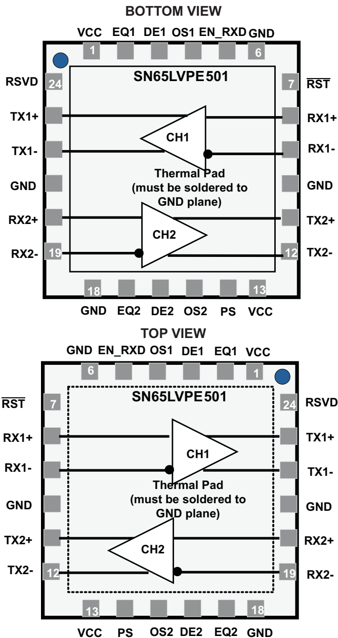
Figure 5. Flow-Through Pin-Out
