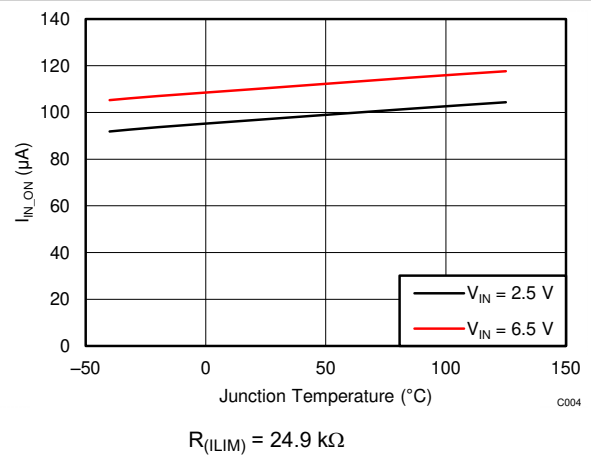
图 7-8. Supply Current, Output Enabled ( I_{IN\_ON} ) vs Temperature
