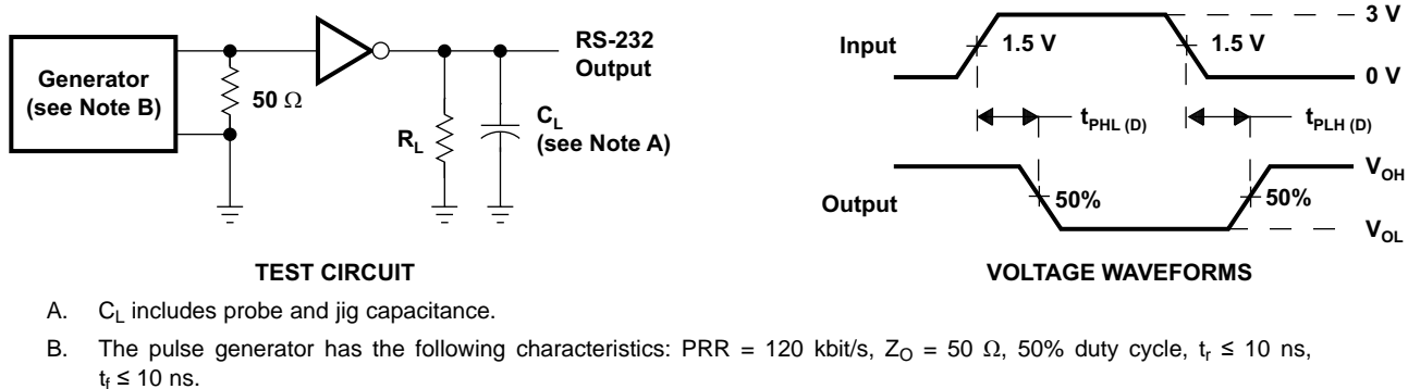
Figure 7. Driver Pulse Skew
