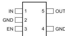
TPS783xxDDC SOT-5 (Top View)
