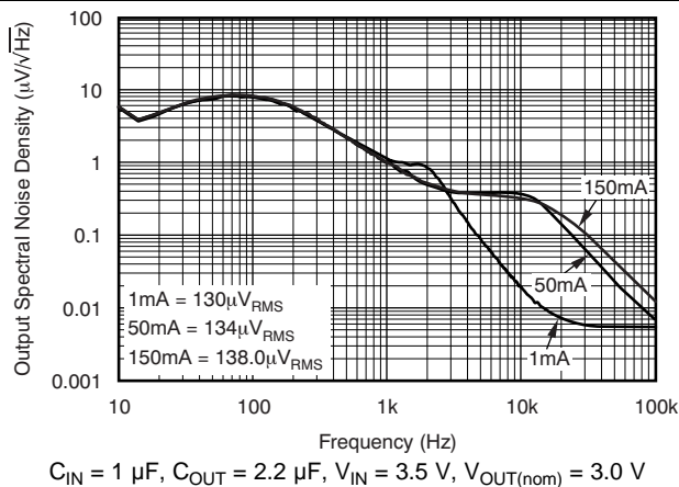
Figure 20. TPS78330 Output Spectral Noise Density
