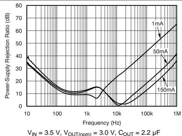
Figure 21. TPS78330 Ripple Rejection vs Frequency
