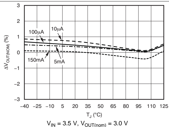
Figure 12. TPS78330 % \Delta V_O vs Junction Temperature
