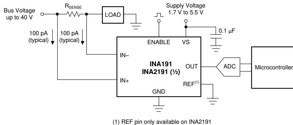
图 8-1. Basic Connections for the INAx191
