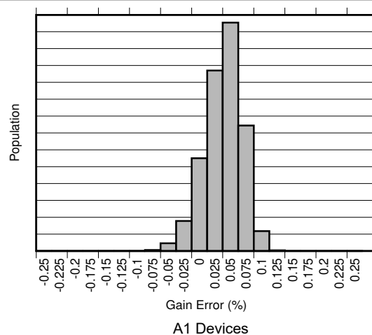
图 6-6. Gain Error Production Distribution (INA2191)
