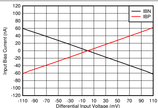
图 6-33. IB+ and IB- vs. Differential Input Voltage (INA191)
