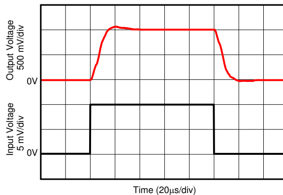
图 6-26. Step Response
