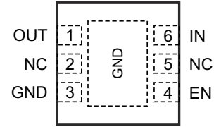
图 5-4. DRV Package, 6-Pin WSON, Top View
