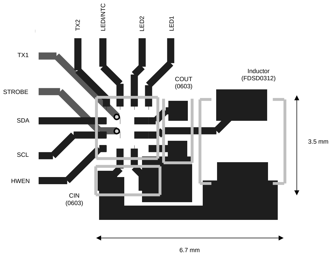
Figure 48. LM3560 Layout
