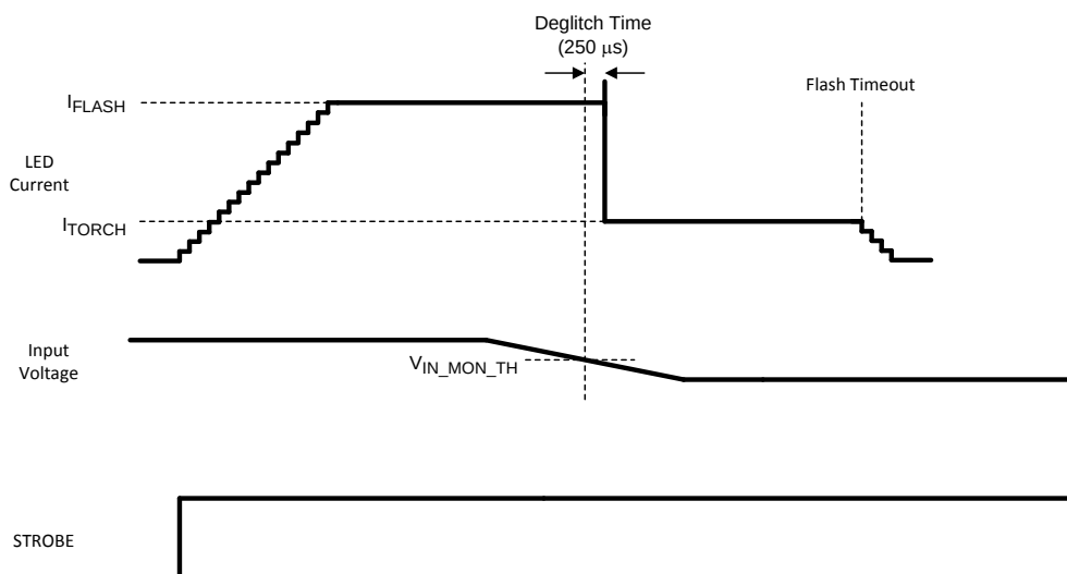
Figure 26. V_{\text{IN}} Monitor Waveform
