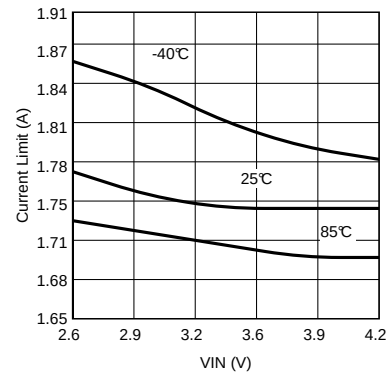
Figure 20. Closed Loop Current Limit vs V_{IN}
