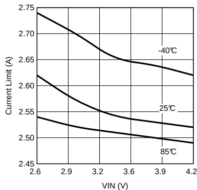
Figure 19. Closed Loop Current Limit vs V_{IN}
