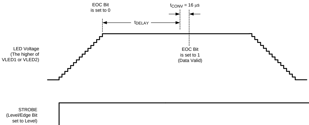
Figure 29. V_{LED} Monitor Automatic Mode
