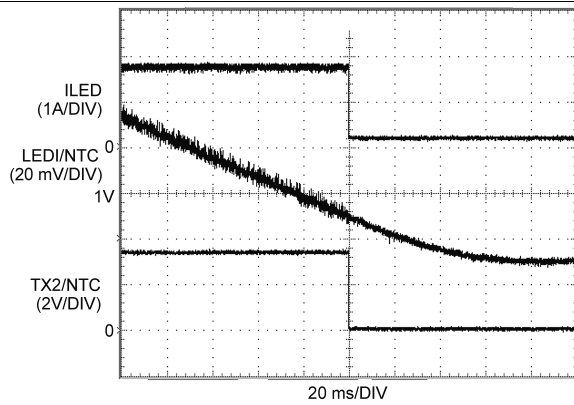
TX2 Set for Interrupt Output (INT) R_3 = 1.3\text{ k}\Omega Circuit of Figure 42 R_{NTC} = 10\text{ k}\Omega at 25^\circ\text{C} NTC Set to Force Torch Mode \text{Beta} = 3380\text{ k}
