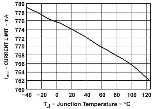
Figure 10. Current Limit vs Temperature
