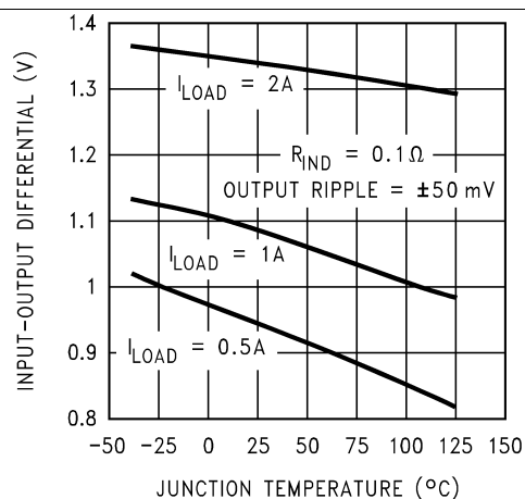
Figure 6. Dropout Voltage
