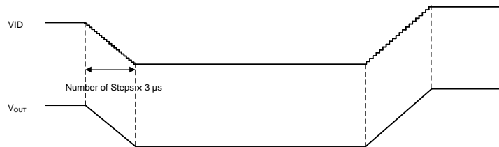
Figure 6-5. DVS Timing Diagram I
