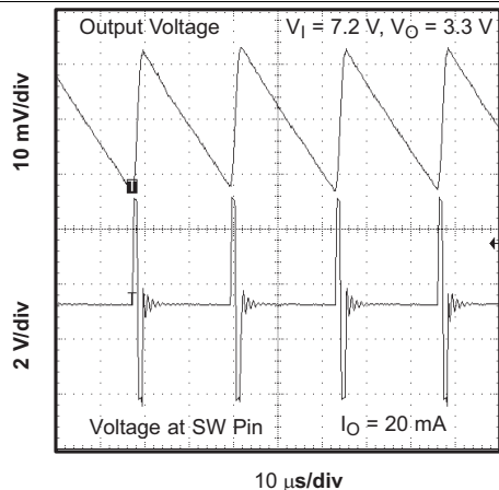
Figure 14. Output Voltage Ripple in Skip Mode
