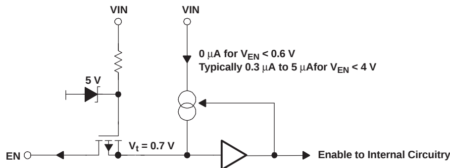
Figure 2. Internal Circuit of the ENABLE Pin
