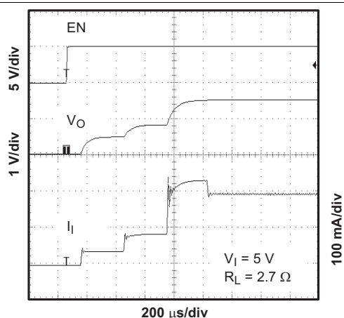
Figure 19. Start-up Timing
