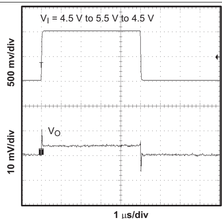
Figure 16. Line Transient Response in PWM Mode
