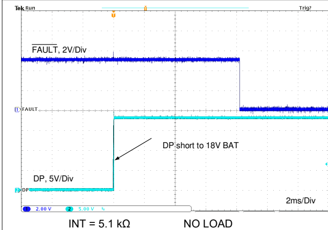
图 11-30. DP Short to BAT
