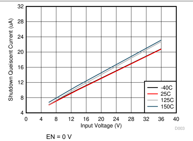
图 8-2. Shutdown Quiescent Current
