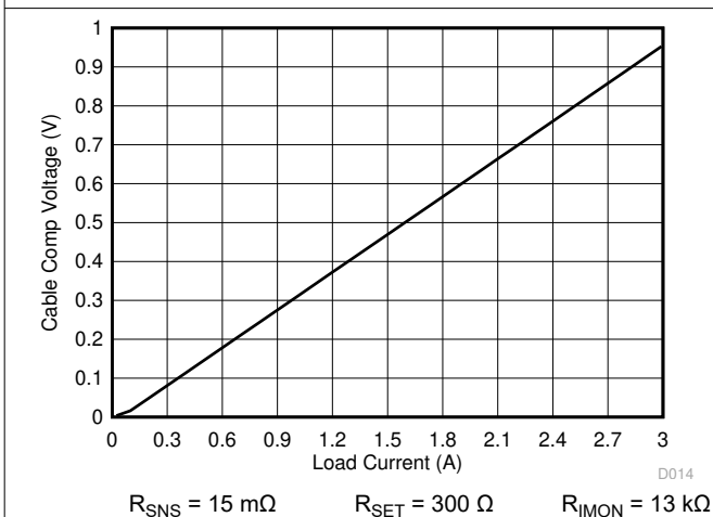
图 8-17. Cable Compensation Voltage vs Load Current
