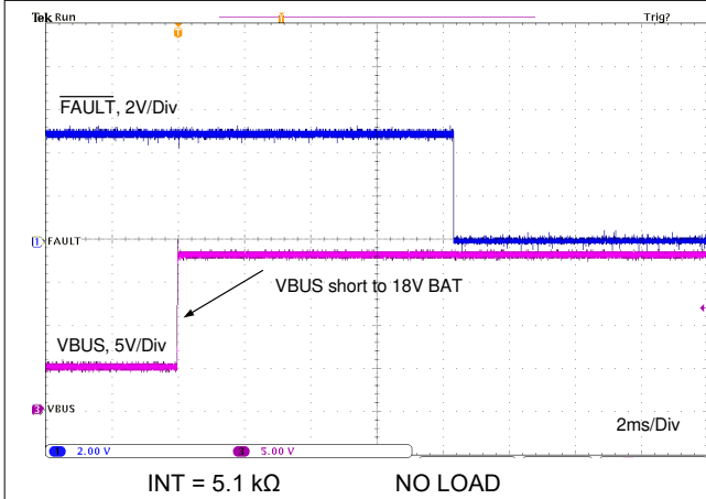
图 11-28. VBUS Short to BAT With External FET
