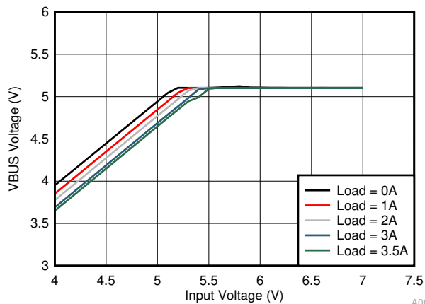
图 11-12. Dropout Characteristic
