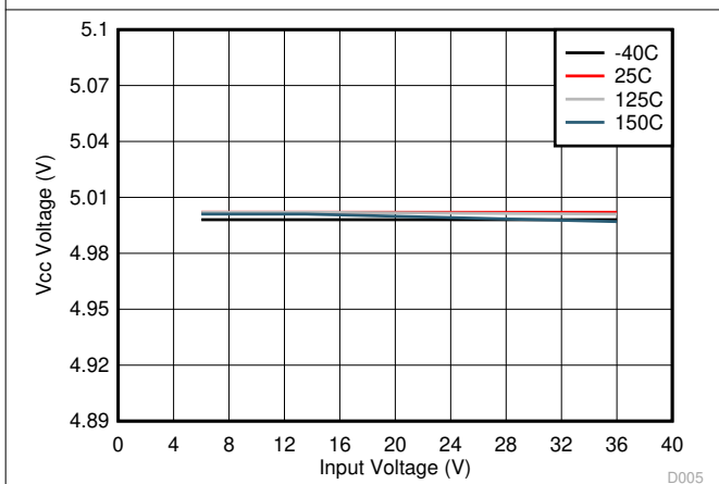
图 8-5. VCC vs Input Voltage
