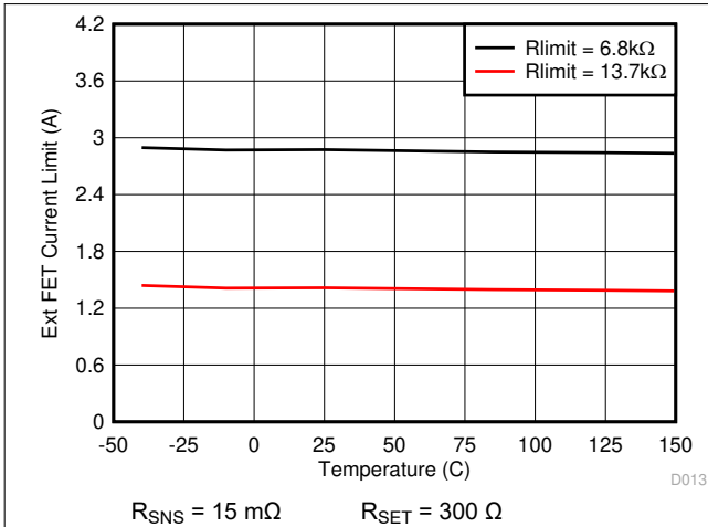
图 8-13. External FET Current Limit vs Junction Temperature
