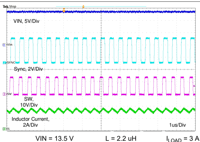
图 10-12. Synchronizing to External 2.1-MHz Clock
