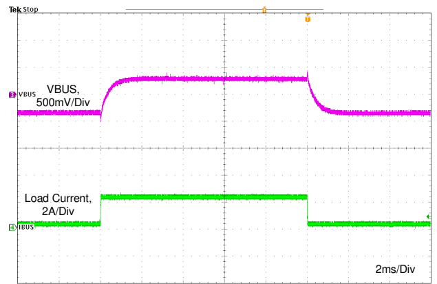
图 11-9. Load Transient Without Cable Compensation
