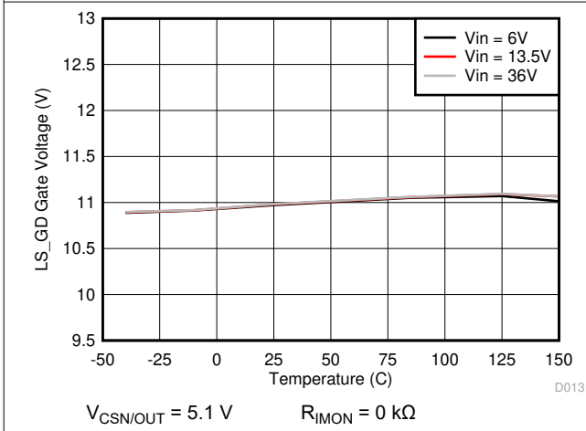
图 8-15. LS_GD Gate Voltage vs Junction Temperature
