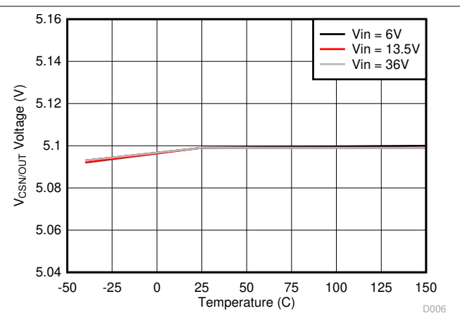
图 8-6. V_{CSN/OUT} Voltage vs Junction Temperature
