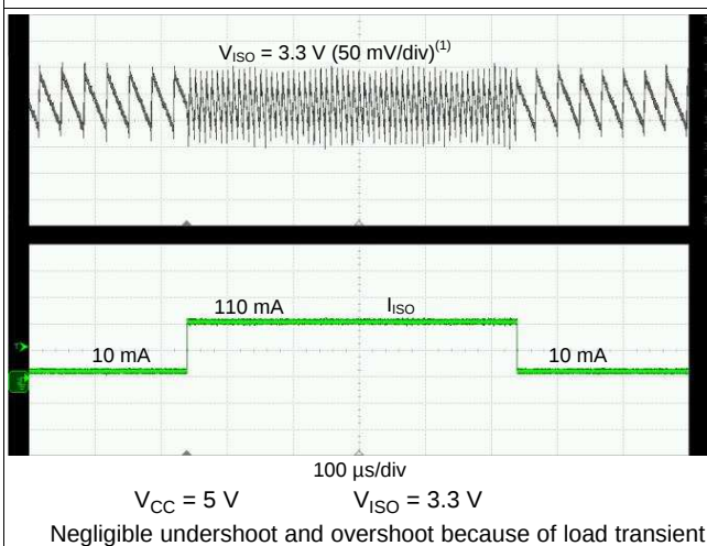
图 25. 10-mA to 110-mA Load Transient Response
