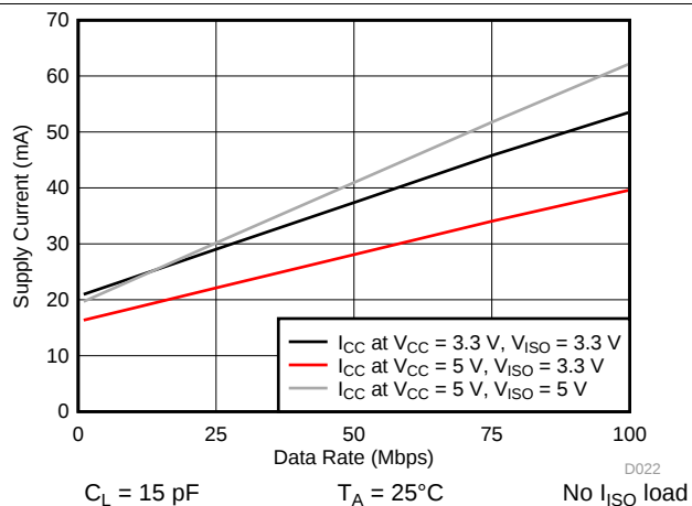
图 11. ISOW7840 Supply Current vs Data Rate
