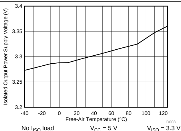
图 8. 3.3-V Isolated Supply Voltage ( V_{ISO} ) vs Free-Air Temperature
