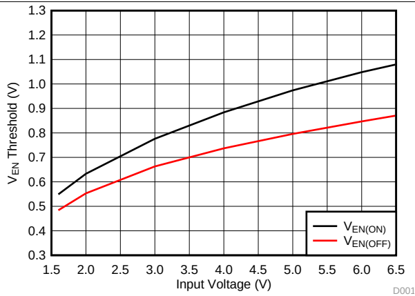
Figure 1. V_{EN} Thresholds vs Input Voltage
