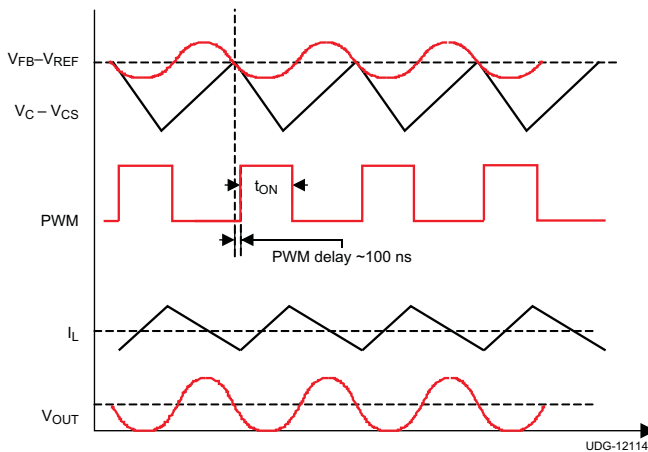
Figure 7. Steady-State Operation
