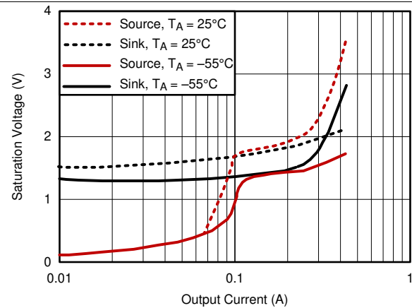
Figure 8. Output Saturation
