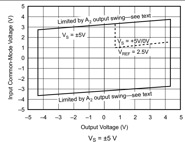
图 6-6. Input Common-Mode Voltage Range vs Output Voltage
