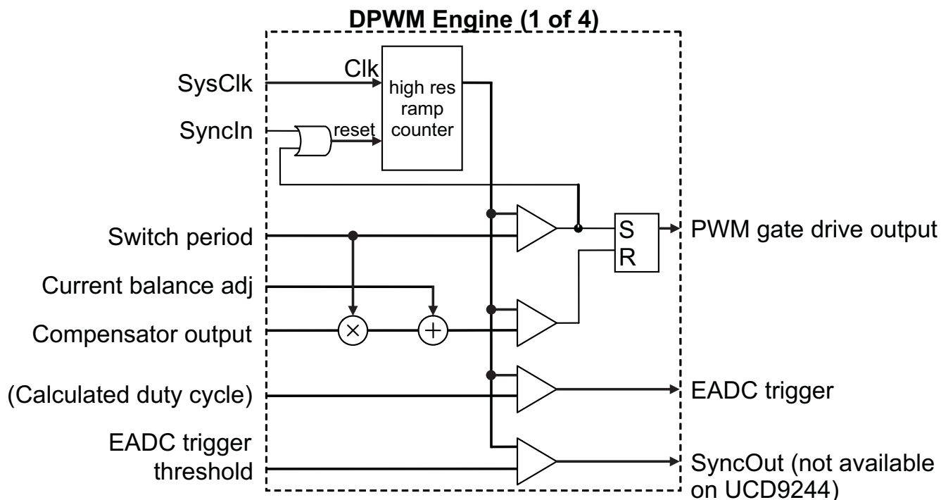
Figure 14. DPWM Engine
