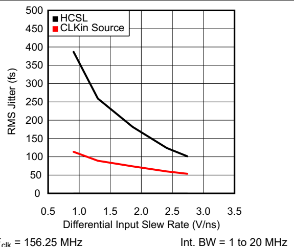
图 6-6. RMS Jitter vs. CLKin Slew Rate at 156.25 MHz
