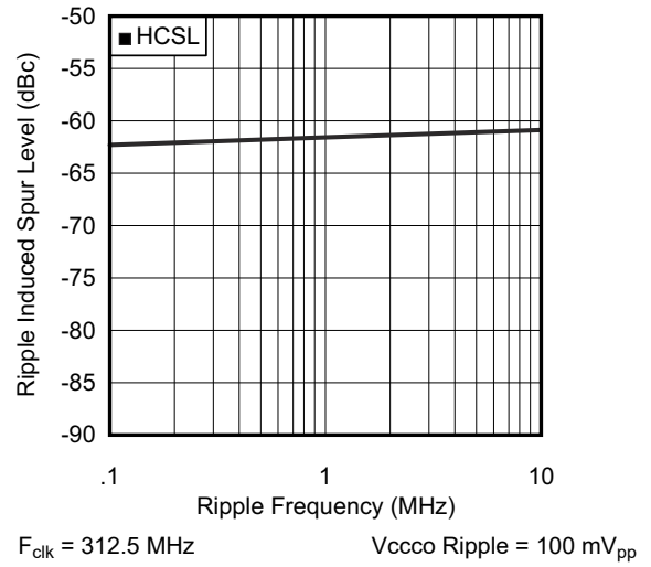
图 6-8. PSRR vs. Ripple Frequency at 312.5 MHz
