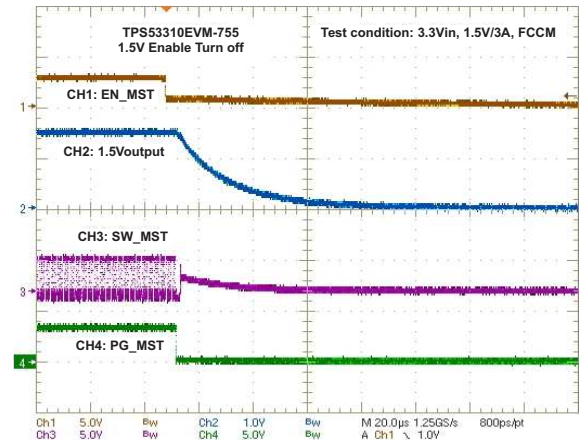
Figure 25. 1.5-V Turnoff Waveform (3.3 VIN, 1.5 V/3 A)
