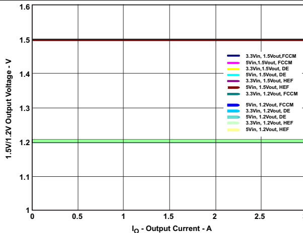
Figure 19. Load Regulation
