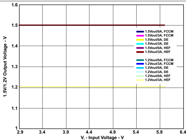
Figure 20. Line Regulation
