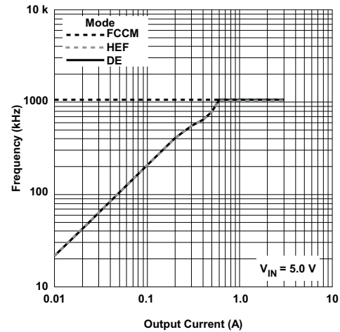
Figure 8. Frequency vs Output Current at V_{IN} = 5 V
