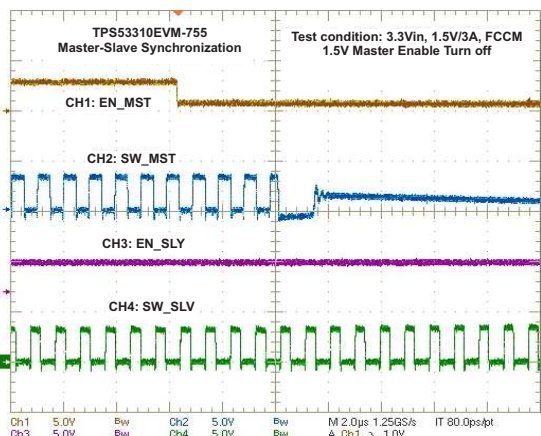
Figure 22. 1.5-V Master Turnoff During Master-Slave Synchronization (3.3 VIN, 1.5 V/3 A, 1.2 V/3 A 180° Synchronization, Then Turn Off Master)
