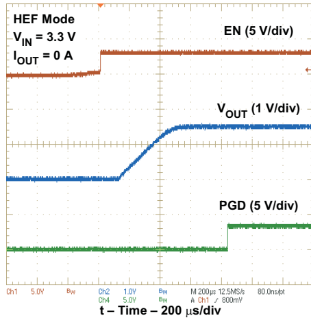
Figure 9. Normal Start Up Waveform
