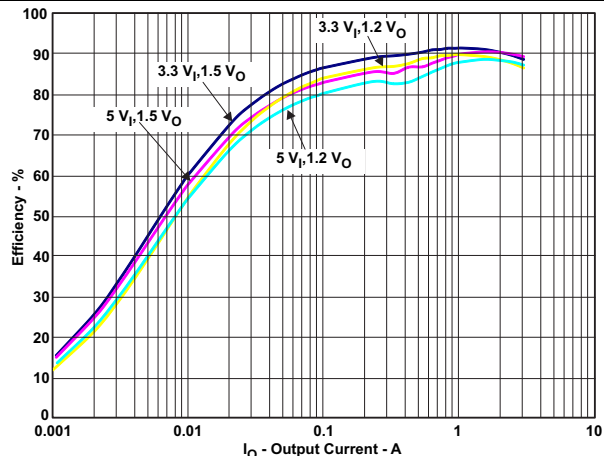
Figure 18. Efficiency
