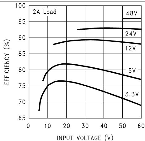
Figure 3. Efficiency
