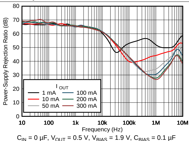
图 26. PSRR vs Frequency and I_{OUT}
