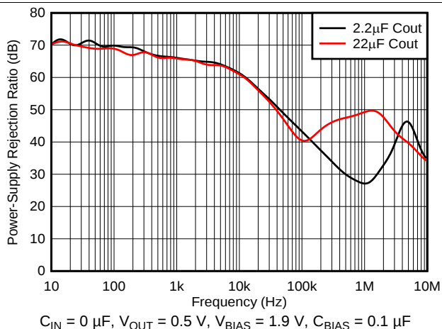
图 28. PSRR vs Frequency and C_{OUT}
