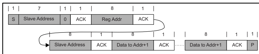
图 25. Multi-Write
