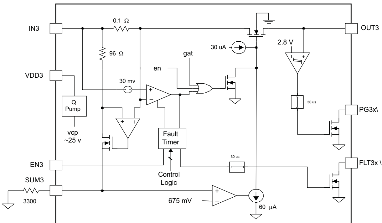
Figure 2. 3-V Channel Circuitry
