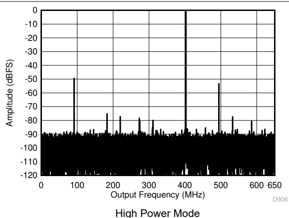
图 7-10. Single Tone FFT at 3497 MHz and -1 dBFS
