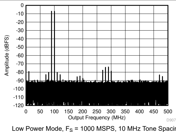
图 7-54. Two Tone FFT at 95.07 MHz Center
