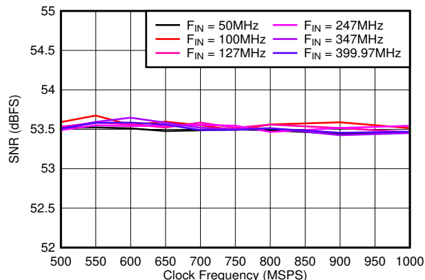
图 7-26. SNR vs Sample Rate
