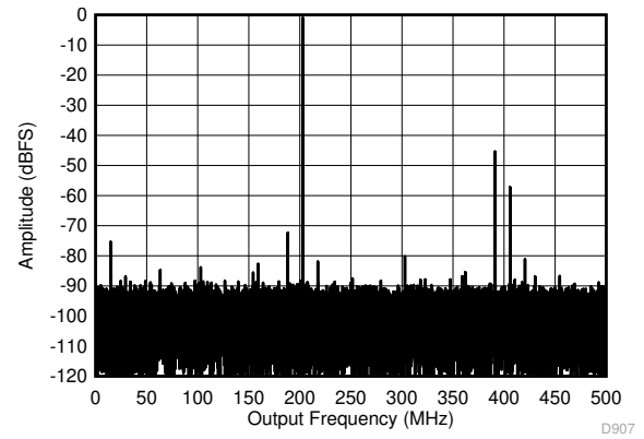
图 7-14. Single Tone FFT at 1797 MHz and -1 dBFS
