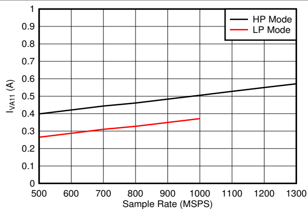
图 7-86. Quad Channel, I_{VA11} vs FS
