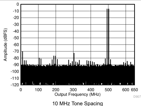
图 7-50. Two Tone FFT at 498 MHz Center
