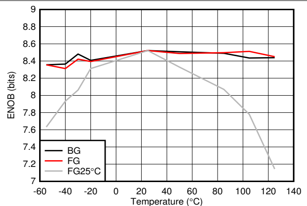
图 7-42. ENOB vs Temperature and Calibration Mode
