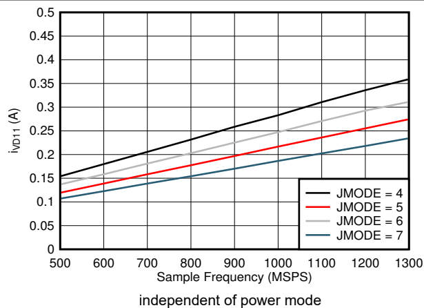
图 7-98. Dual Channel, I_{VD11} vs FS and JMODE 4 - 7
