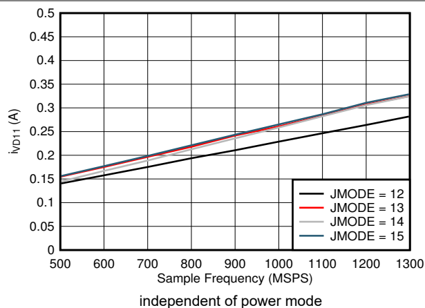
图 7-100. Dual Channel, I_{VD11} vs FS and JMODE 12 - 15
