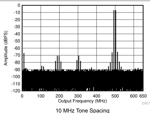
图 7-52. Two Tone FFT at 1798 MHz Center
