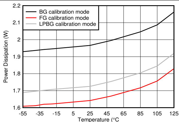
图 7-124. Dual Channel, Power Dissipation vs Temperature
