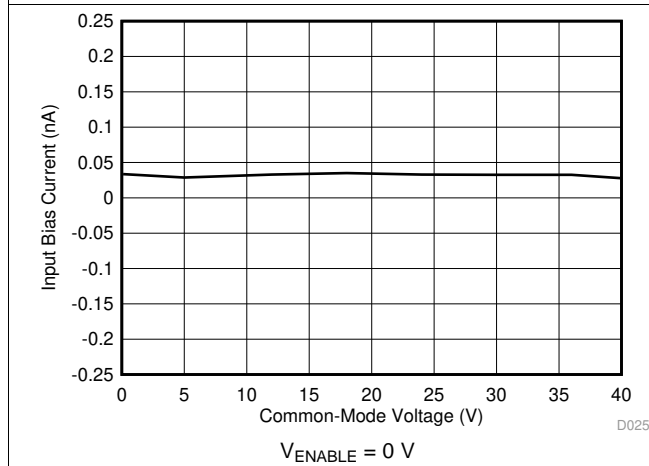
图 15. Input Bias Current vs Common-Mode Voltage (Shutdown)
