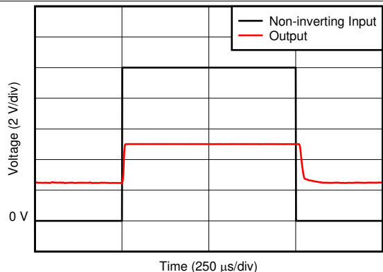
图 25. Noninverting Differential Input Overload
