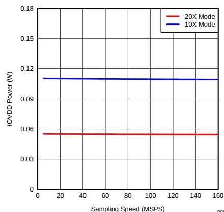
图 41. Analog Power vs Sampling Frequency
