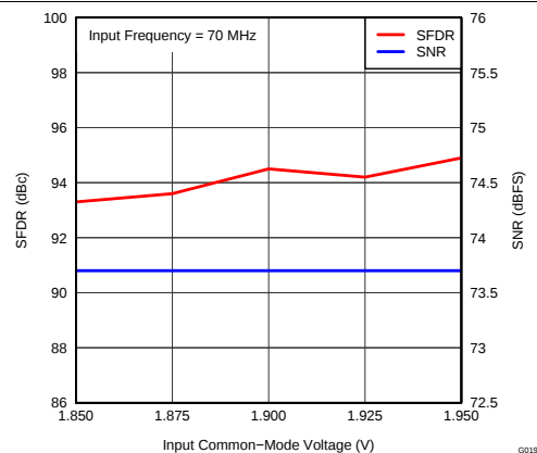
图 24. Performance vs Input Common-Mode Voltage (70 MHz)
