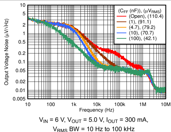
图 6-74. Output Noise vs Frequency and C_{FF}
