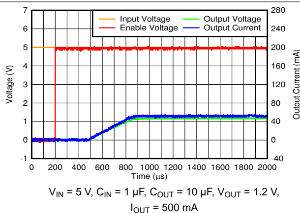
图 6-78. Start Up at -40^\circ\text{C}
