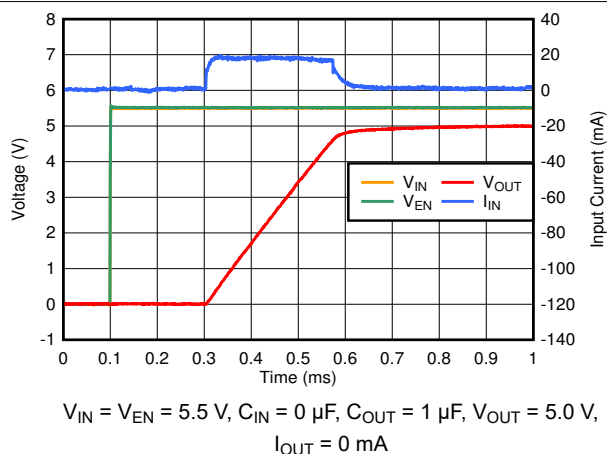
图 6-76. Start-Up Inrush Current With C_{OUT} = 1\text{ }\mu\text{F}
