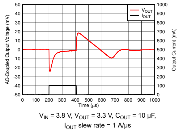
图 8-10. I_{OUT} Transient From 1 mA to 100 mA
