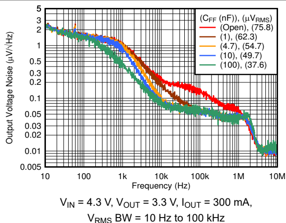
图 6-73. Output Noise vs Frequency and C_{FF}
