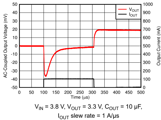
图 8-9. I_{OUT} Transient From 0 mA to 100 mA
