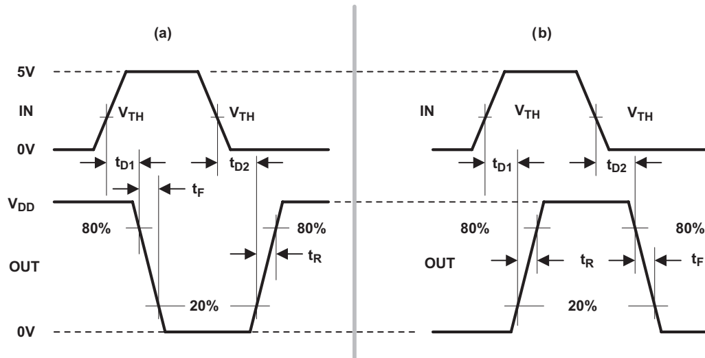
Figure 1. Switching Waveforms for (a) Inverting Input to (b) Output Times
