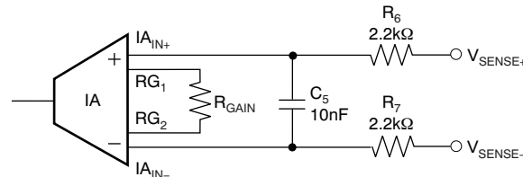
Figure 44. Current-Limiting Resistors
