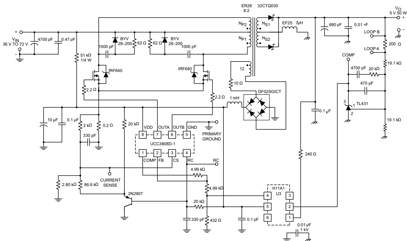
Figure 6. Typical Application Diagram: 48-V In, 5-V, 50-W Output
