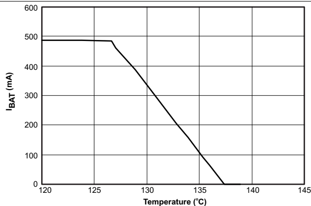
Figure 1. Thermal Regulation
