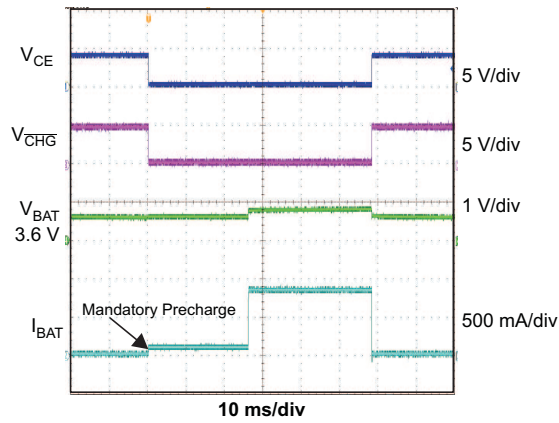
Figure 33. Charger ON/OFF Using \overline{\text{CE}}
