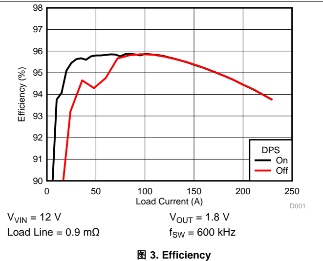
图 3. Efficiency
