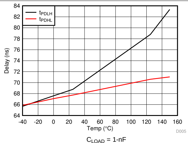
图 7. Propagation delay versus Temperature
