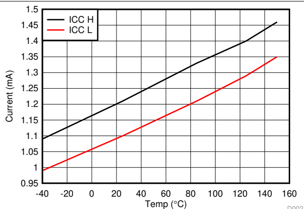
图 4. Supply currents versus Temperature
