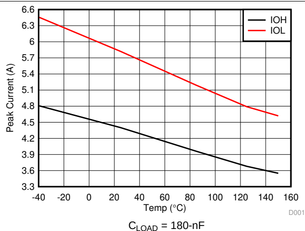
图 3. Output Drive currents versus Temperature
