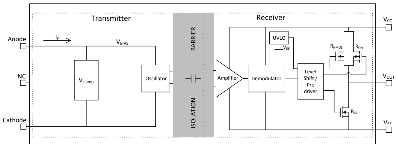
图 19. Conceptual Block Diagram of a Isolated Gate Driver with an Opto Emulated Input Stage (SO6 pkg)
