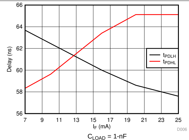
图 8. Propagation delay versus Forward current
