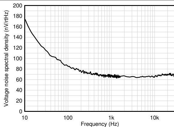
图 7-22. Input Voltage Noise Spectral Density
