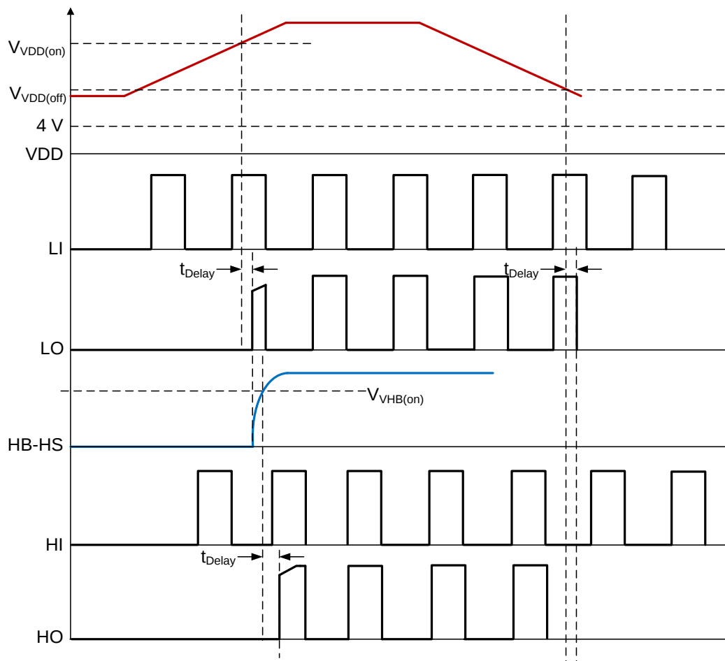
图 30. Power-Up Driver
