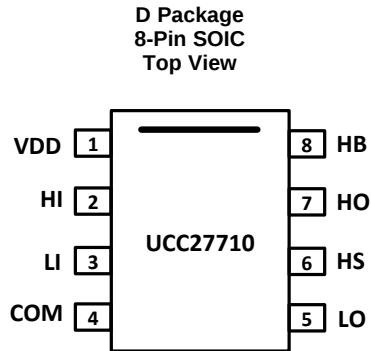
Pin Functions
