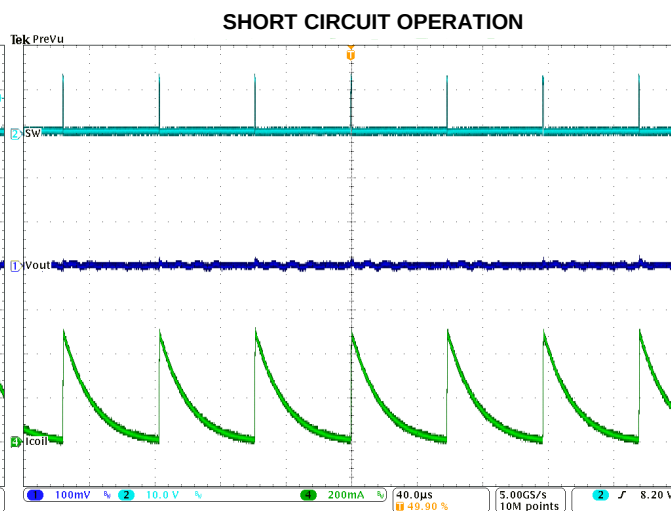
Figure 52. Short circuit from startup, V_{IN}=12V
