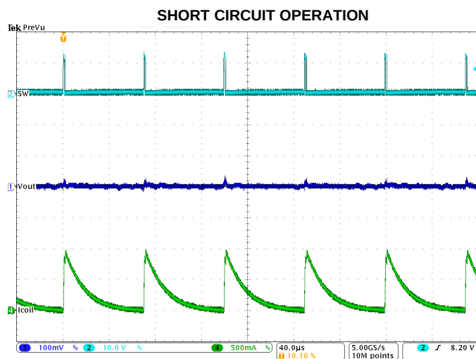
Figure 51. Short circuit while running, V_{IN}=12V
