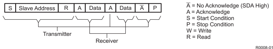
Figure 56. I 2 C Read Cycle
